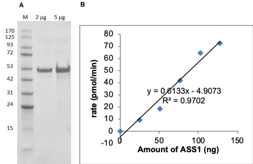
Fig A. SDS-PAGE (4-20%) recombinant ASS1: Recombinant protein loaded under reducing conditions and stained with Coomassie Blue. Lane M-MW marker
