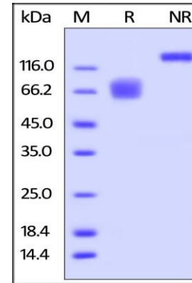
Human CD58, Fc Tag on SDS-PAGE under reducing (R) and no-reducing (NR) conditions
