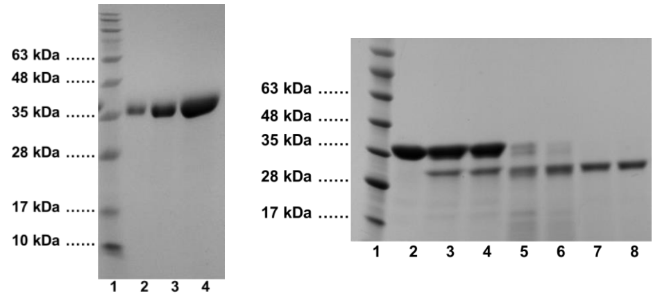
SDS-PAGE (15%) of h-Procathepsin B: 1: Protein Marker 2: Human Procathepsin B (5 µg) 3: Human Procathepsin B (10 µg) 4: Human Procathepsin B (20 µg) SDS-PAGE (15%) of activation of h-Procathepsin B: 1: Protein Marker 2: Human Procathepsin B (10 µg) 3 to 8: Human Procathepsin B (10 µg) after 0.5, 1, 2, 3, 4 and 5 h of activation at pH 4.0
