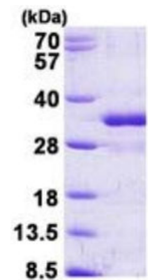
15% SDS-PAGE (3µg) FGF14, human recombinant
