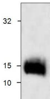
Western blot analysis of IL-21 using recombinant human IL-21
