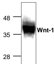
Cat. #: 4754-10 Purity of recombinant Wnt-1 (2 µg) was analyzed by reduced SDS-PAGE electrophoresis.
