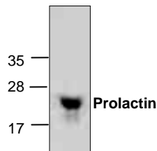
Cat. #: 4688-50 Purity of recombinant murine Prolactin (2 µg) was analyzed by reduced SDS-PAGE electrophoresis.
