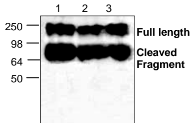
Cat. #: 3697-100 Western blot analysis of Dicer expression in Jurkat cell lysate (Lane 1 & 2) and mouse small intestine tissue lysate (Lane 3).
