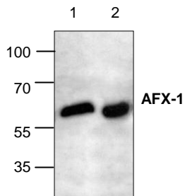
Cat #: 3404-100 Western blot analysis of FOXO4/AFX1 in 3T3 cell lysate (Lane 1) and rat kidney tissue lysate (Lane 2).
