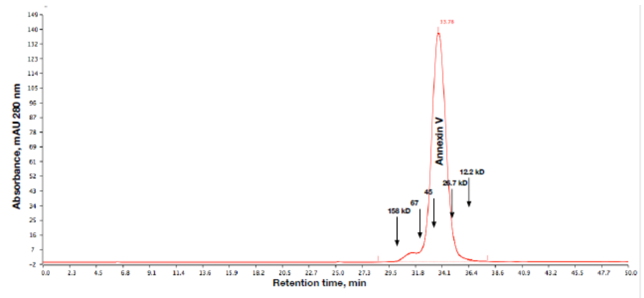
Analytical Size Exclusion Chromatography run of Annexin V
