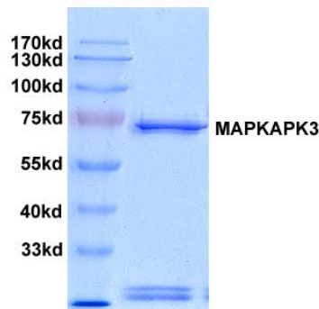
Fig. 2 MAPKAPK3 protein gel
