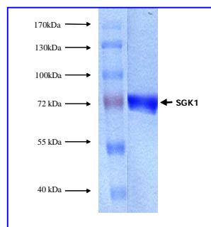
Fig. 1 SGK1 protein gel
