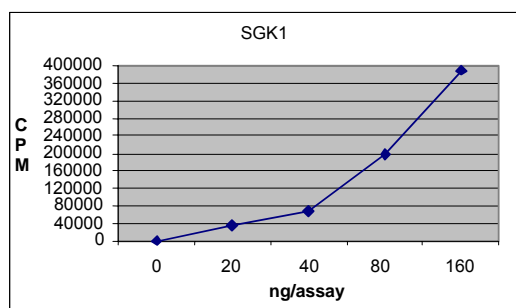
Fig. 1 SGK1 activity assay
