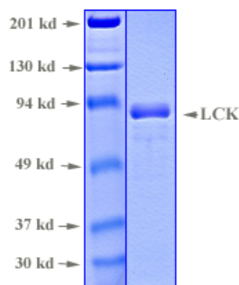
Fig. 2 LCK protein gel
