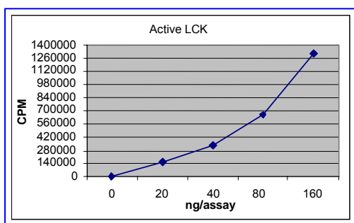
Fig. 1 LCK activity assay
