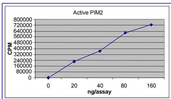
Fig. 1 Pim2 activity assay
