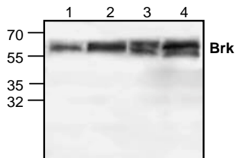
Cat. #:3847-100 Western blot analysis of Brk in lysates from Jurkat cells (Lane 1,2), 3T3 cells (Lane 3) and rat kidney (Lane 4).
