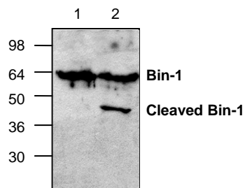
Cat.# 3672-100 Western blot analysis of BIN-1 expression in Jurkat cells treated with (Lane 2) or without (Lane 1) camptothecin.
