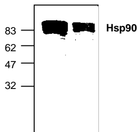
Cat.# 3389-100 Western blot analysis of Hsp90 expression in Jurkat cell lysate (Lane 1) and mouse small intestine tissue lysate (lane 2).
