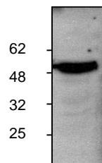
Western blot analysis of PBR expression in rat kidney tissue lysate.
